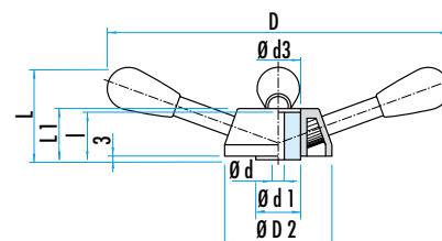
Ref. EWN.VBR.4
