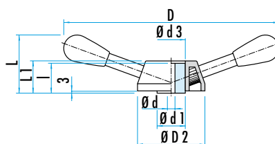
Ref. EWN.VBR.2
