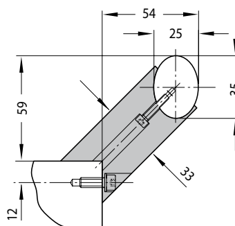
RSC.U4.25 verticale montage
